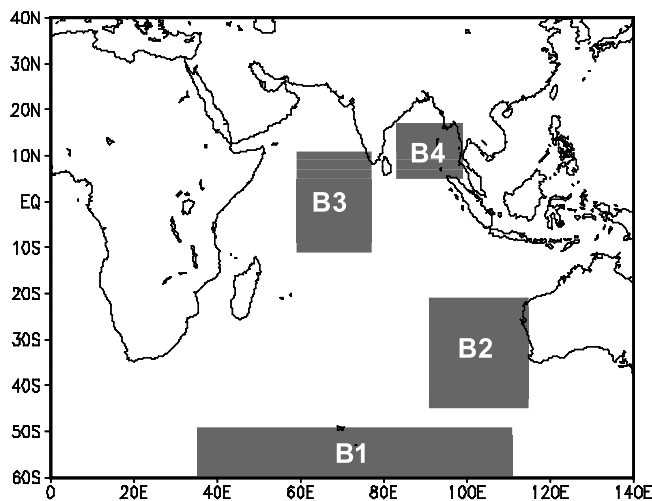
Figure 4. Oceanic region sites at middle latitudes of the South Indian Ocean (B1), to southwest of Australia (B2), in the equatorial Indian Ocean (B3), and in the Bay of Bengal (B4).
