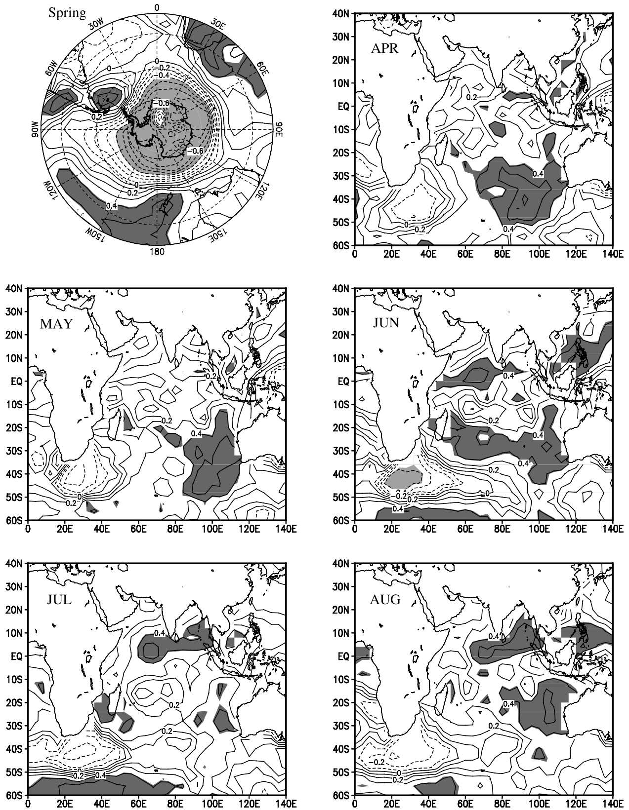
Figure 2. Heterogeneous correlation patterns of the leading ESVD mode for the spring (April–May) SH SLP anomalies south of 10°S (top left) and the Indian Ocean SST anomalies from April to August, respectively. The areas with positive (negative) correlation coefficients that are significant at the 99% confidence level are shaded dark (light). The latitude lines in the top left are at a 20-degree interval starting from 1°
