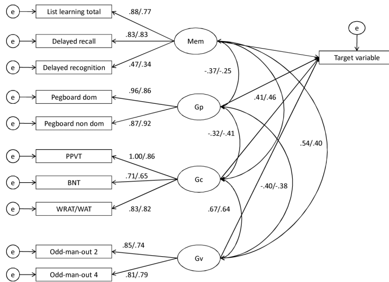
Figure 1. Representation of the four-factor structural model (Model B) comprises memory, Gp, Gc, and Gv constructs. Two-headed arrows connecting latent variables (depicted as circles) represent correlations between the constructs. The paths from the latent constructs to the observed variables (depicted as rectangles) represent the loadings of each task onto its respective construct. The values presented represent the standardized path coefficients for the lower order loadings, and the inter-factor correlations. The first number represents the value for the English speaking sample and the second number represents the value for the Spanish speaking sample. All the loadings and inter-factor correlations are significant at the p < .01 level. The latent variables labeled “e” represent the unique variance and error associated with each observed variable.
