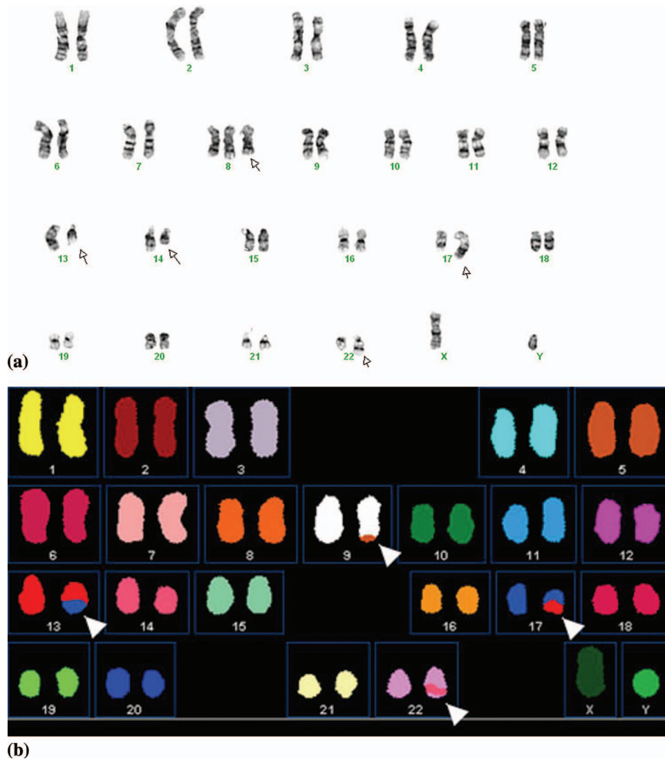
Figure 1. (a) A G-banded karyotype showing 46,XY, +8,t(13;17)(q12;q22),t(14;22)(q23;q13). Arrows indicate abnormal chromosomes. (b) A SKY karyotype showing 47,XY, +8,der(9)t(5;9)(?;q34),t(13;17)(q12;q22),del(14)(q23),ins(22;14)(q13.1;q24q32). Abnormalities are indicated.
