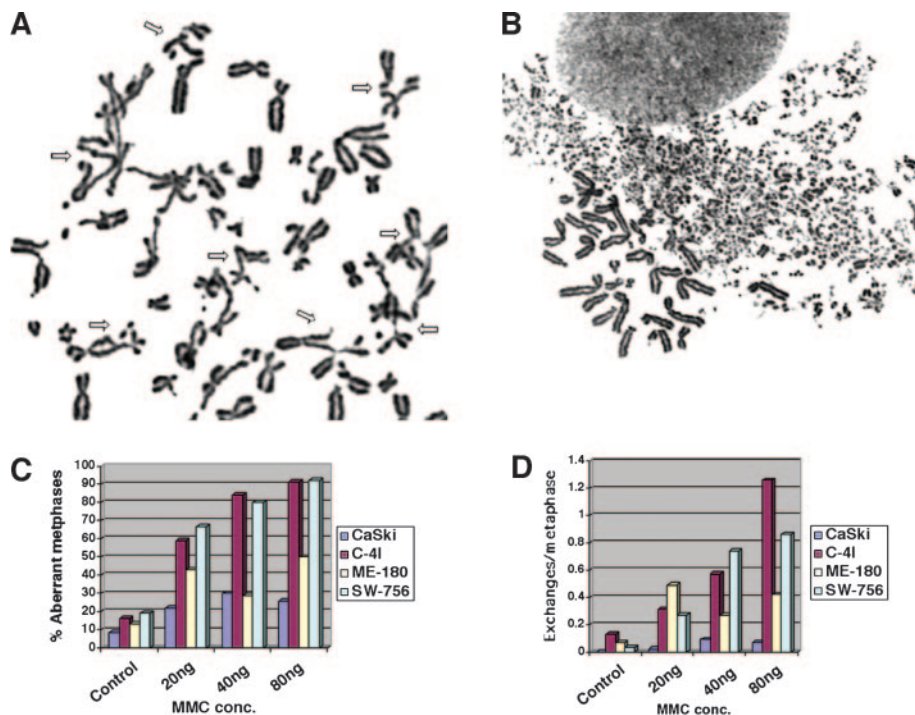
Fig. 4. FANCF inactivated cervical cancer cell lines are hypersensitive to mitomycin C (MMC) treatment. A , MMC-induced chromosome breakage in SW756 cell line. A representative micrograph showing chromosome radials (arrows). B , a near tetraploid metaphase from C-4I cell line showing MMC-induced multiple breakages. C and D , MMC-induced chromosomal aberrations in FANCF -inactivated cell lines. Percentage of aberrant metaphases with all types of aberrations ( C ) and multiradials/metaphase ( D ) are shown. The cell line CaSki had no evidence of FANCF defect. C-4I cell line showed no evidence of FANCF promoter methylation but exhibited down-regulated expression and activation by treatment with TSA. ME-180 and SW756 cell lines had FANCF promoter hypermethylation and down-regulated expression.
