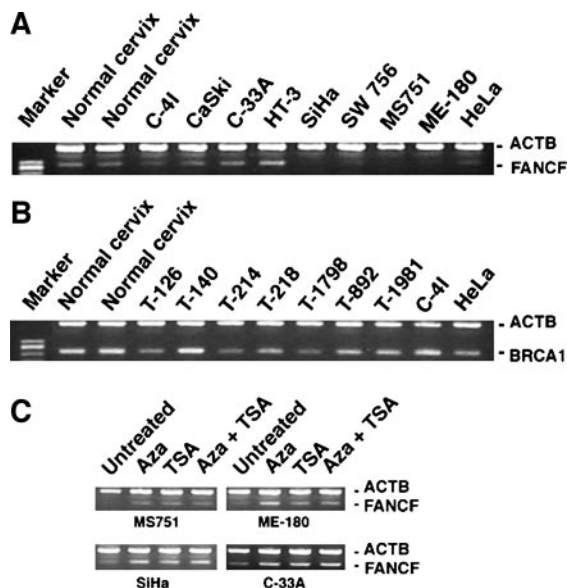
Fig. 2. Semiquantitative analysis of FANCF and BRCA1 expression by reverse transcription-PCR in cervical cancer cell lines and primary tumors. ACTB , \beta -actin; T, primary tumor; A, FANCF expression in CC. Because FANCF coding region spans in a single exon, we treated the total RNA with two rounds of DNase to avoid amplifying contaminating DNA. Note the down-regulated expression of FANCF in the cell lines C-4I, SiHa, SW756, MS751, ME-180, and HeLa. B, BRCA1 expression in CC. Decreased levels of BRCA1 expression was found in T-126, T-214, and T-1798. C, effect of demethylation and acetylation on FANCF gene expression. Two rounds of DNase treated total RNA was used in reverse transcription reactions to avoid amplifying contaminating DNA.
