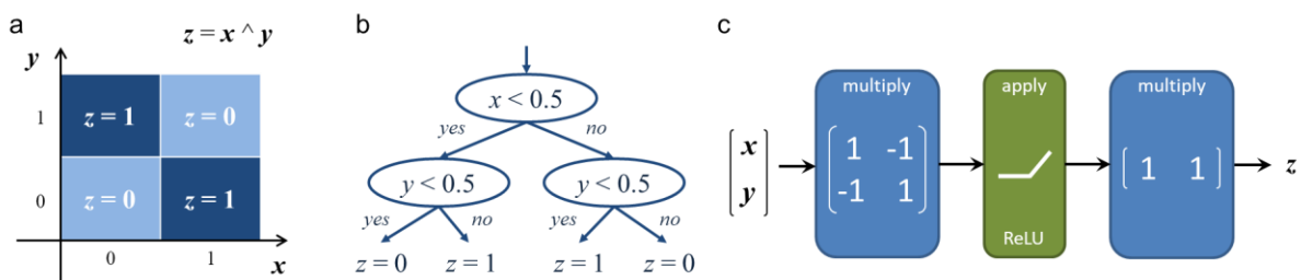
Figure 1.3: (a) The XOR function, z = x \wedge y . (b) The decision tree approach towards the XOR function. (c) The neural network approach towards the XOR function. The ReLU function is defined as \text{ReLU}(x) = x, x > 0; 0, x \leq 0 .
