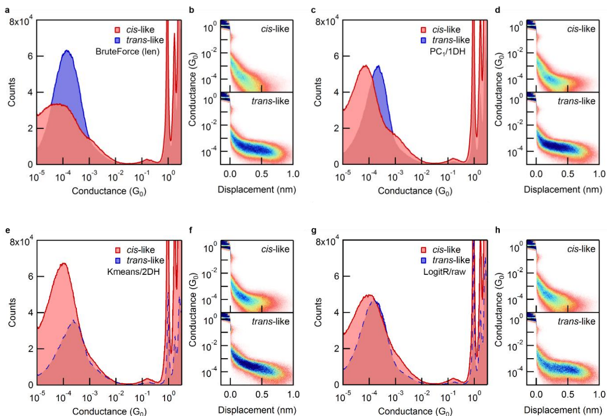
Figure 3.10: Histograms of the traces judged to be 4-like or 5-like from the traces measured after ~22 hrs starting with a pure 4 solution. (a) The 1D and (b) 2D histograms classified by the brute force model: there are 5,653 cis -like (4-like) traces and 4,338 trans -like (5-like) traces; here the brute force model judges based on counts of points in the molecular conductance region. (c) The 1D and (d) 2D histograms classified by the PC_1/1DH model: there are 6,577 cis -like traces and 3,414 trans -like traces. (e) The 1D and (f) 2D histograms classified by the KMeans/2DH model: there are 7,552 cis -like traces and 2,439 trans -like traces. (g) The 1D and (h) 2D histograms classified by the logistic regression model on raw traces: there are 6,691 cis -like traces and 3,300 trans -like traces.
