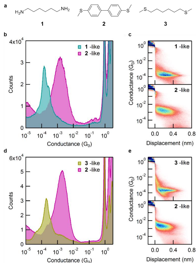
Figure 3.3: (a) Chemical structures of 1, 2, 3. (b) The 1D and (c) 2D histograms of the traces judged to be 1-like (3,406 traces) or 2-like (4,876 traces) by the CNN model from mixed solution measurements. The histograms of all traces are shown in Figure 3.1b and 3.1c, and histograms of measurements on pure solutions are shown in Figure 3.6. (d) The 1D and (e) 2D histograms of the traces judged to be 2-like (7,678 traces) or 3-like (4,098 traces) by the CNN model from mixed solution measurements.
