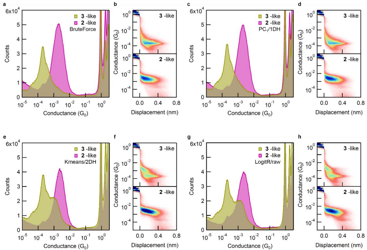
Figure 3.9: Histograms of the traces judged to be 2-like or 3-like from measurements of a mixed solution. (a) The 1D and (b) 2D histograms classified by the brute force model: there are 7,062 2-like traces and 4,737 3-like traces. (c) The 1D and (d) 2D histograms classified by the PC 1 /1DH model: there are 6,549 2-like traces and 5,250 3-like traces. (e) The 1D and (f) 2D histograms classified by the KMeans/2DH model: there are 4,625 2-like traces and 7,151 3-like traces. (g) The 1D and (h) 2D histograms classified by the logistic regression model on raw traces: there are 4,959 2-like traces and 6,817 3-like traces.
