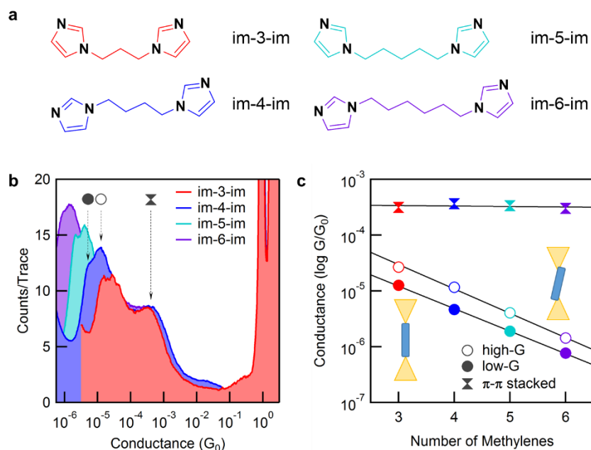
Figure 2.2: (a) The chemical structures of im-N-im molecules. (b) Logarithmically-binned conductance histograms (100 bins per decade) for all four molecules generated from 15000 traces each. The three peaks, two that change with the molecular backbone length and the one that is independent of the backbone length are indicated by the arrows for im-4-im. Histograms are terminated at the noise floor. (c) Molecular junction conductance, determined from a Gaussian fit, is plotted against the number of methylene units in the backbone. The \beta values determined from the fit are 0.93 (low-G) and 1.01 (high-G), per methylene.
