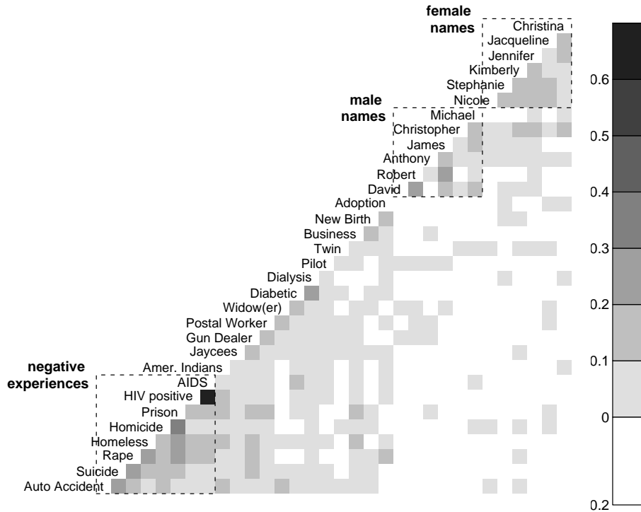
Figure 8: Correlations of the residuals r_{ik} among the survey respondents: people who know more HIV-positive persons know more AIDS patients, etc. The groups other than the names are ordered based on a clustering algorithm that maximizes correlations between nearby groups.
