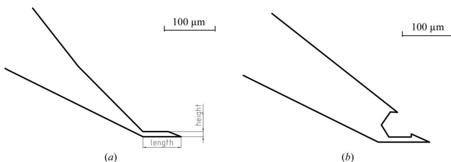
Figure 2 Two different forms of silicon microshovels. (a) Design No. 0, (b) design No. 17A.
