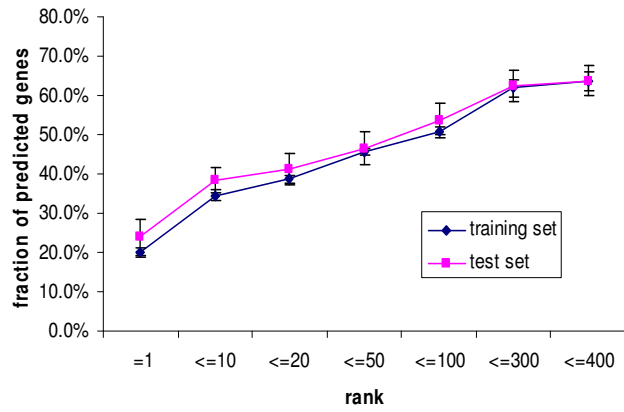
Figure 3. 10-fold cross-validation of the predictive algorithm. Error bars represent the variations in terms of prediction over the sample sets. Similar results were obtained for the training sets and test sets, suggesting overfitting is not a problem of the method.
