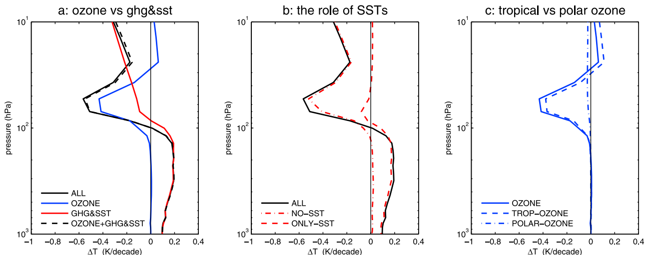
Figure 3. Annual mean model temperature response ( \Delta T ), averaged 30^\circ\text{S} – 30^\circ\text{N} , in K/decade, for different model integrations, as indicated in the legends. The thin, vertical, solid, black line marks the zero response.
