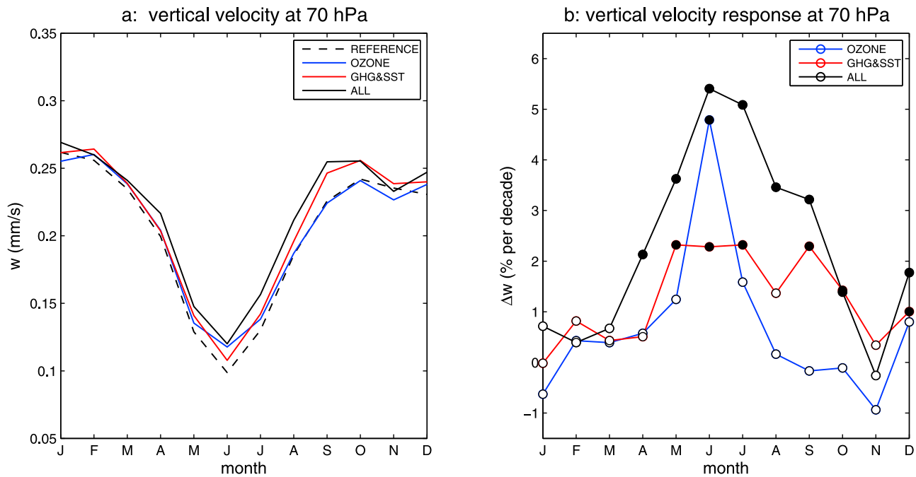
Figure 7. As in Figure 6, but for the seasonal cycle of (a) w and (b) \Delta w , at 70 hPa, averaged 20°S to 20°N.
