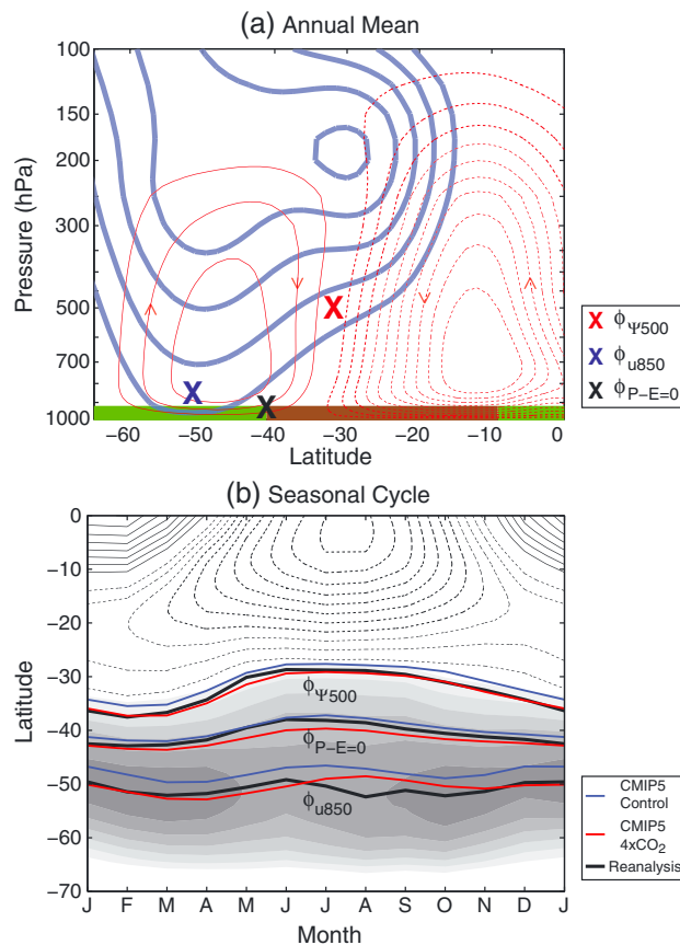
Figure 1. The 1979–2012 ERA-Interim reanalysis zonal mean climatology: (a) annual mean and (b) monthly mean. In Figure 1a, thick blue lines denote zonal mean zonal wind (contour interval: 5 \text{ m s}^{-1} for values \geq 10 \text{ m s}^{-1} ), and thin red lines denote mean meridional mass stream function (contour interval: 1.0 \times 10^{10} \text{ kg s}^{-1} ; negative contours dashed; zero contour omitted). Regions where zonal mean precipitation is greater (less) than zonal mean evaporation are shaded in green (brown). In Figure 1b, gray shading denotes 850 hPa zonal mean zonal wind (contour interval: 2 \text{ m s}^{-1} for values \geq 2 \text{ m s}^{-1} ), and thin black lines denote 500 hPa mean meridional mass stream function (contour interval: 2.0 \times 10^{10} \text{ kg s}^{-1} ; negative contours dashed; zero contour omitted). The locations of \phi_{u850} , \phi_{P-E=0} , and \phi_{\psi500} are indicated for ERA-Interim reanalysis (thick black line), the multimodel mean CMIP5 preindustrial control climatology (blue), and the multimodel mean CMIP5 4 \times \text{CO}_2 climatology (red).
