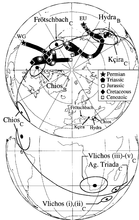
Fig. 9. The paleomagnetic poles from Frötschbach and Hydra (Table 1) and from other regions in the Mediterranean (Chios, Greece, and Kçira, Albania) compared with the West Gondwana (WG, in northwest Africa coordinates) and Europe (EU) apparent polar wander paths [27]. The suffix attached to the pole designation refers to the magnetization component used for pole calculation: C = the characteristic component, B = a secondary component (note that Hydra B is the mean of Vlichos B and Aghia Triada B ). The solid line is a small circle centered on the eastern Mediterranean (28°E, 36°N) whose radius of 78° is approximately the average paleoco-latitude of the Frötschbach and Hydra characteristic and ancient overprint magnetizations, illustrating that vertical axis rotations can account for the dispersion of these paleopoles.
