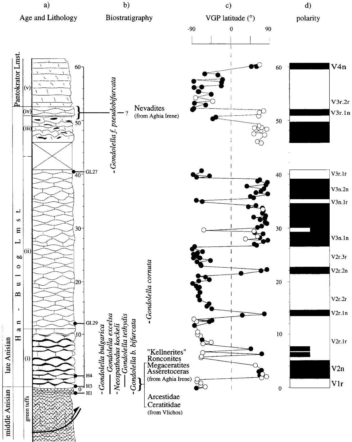
Fig. 6. The middle/late Anisian Vlichos section. For column descriptions see Fig. 2. Conodont biostratigraphy is from [19]. In the VGP latitude column, ○ = mainly hematite, ● = mainly magnetite is the magnetic carrier of the characteristic remanence.
