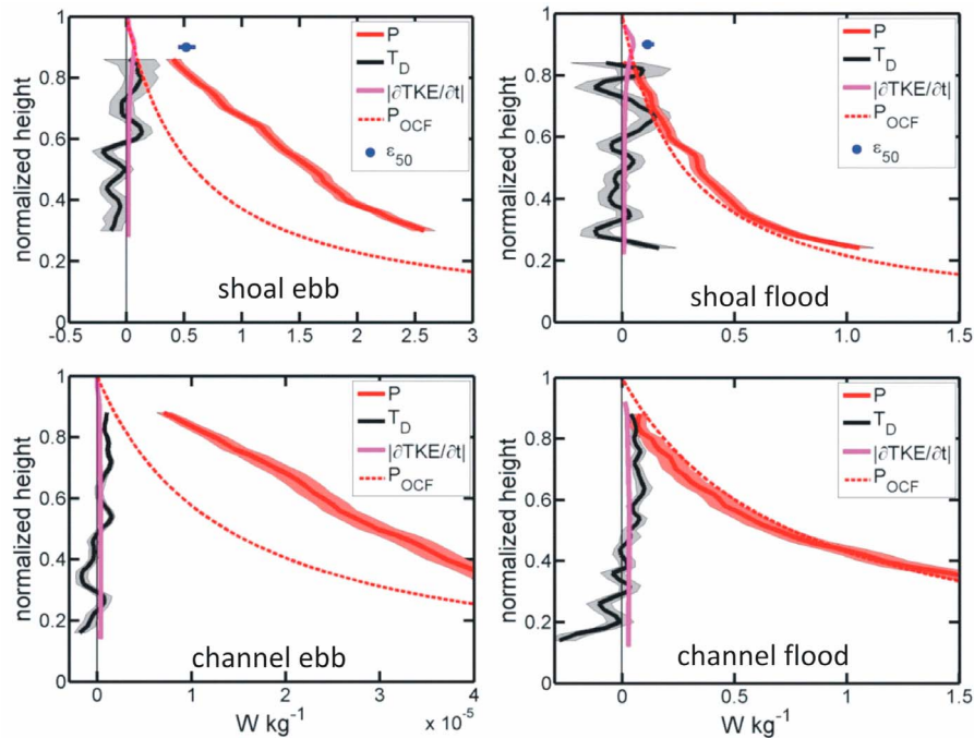
Figure 11. Mean TKE budget terms for strong spring tides with low winds: TKE shear production ( P ), net turbulent TKE flux ( T_D ), mean absolute value of TKE tendency ( \partial TKE/\partial t ), and dissipation at 50 cm depth ( \varepsilon_{50} ) from SOCa (shoal budget only). Observed standard error is shown as shading around T_D and P and as a horizontal line for \varepsilon_{50} . For the shoal site, the near-surface TKE budget is quantified at \sim 50 cm depth as \partial TKE/\partial t = P - 0.2P - \varepsilon + T_D (section 4.2). An open-channel flow model of P is also shown for comparison ( P_{OCF} ).
