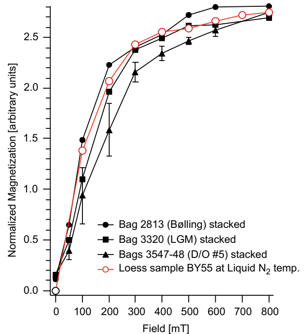
Fig. 6. IRM acquisition curves for North GRIP ice core samples. Each curve represents the stack of several samples from the same climatic interval normalized to unit variance. Error bars of samples from bags 3547–48 (Dansgaard/Oeschger #5 transition) represent the standard deviation ( \pm\sigma ); \sigma in samples from Bølling and Last Glacial Maximum is smaller than symbol size. \text{IRM}_{77\text{K}} acquisition of loess sample BY55 is shown for comparison. The \text{IRM}_{300\text{K}} intensity (at 800 mT) of loess sample BY55 is comparable to that of Greenland ice dust ( 7.5 \pm 2 \text{ mA m}^2/\text{kg} ) as they share the same source area (the Gobi Desert).
