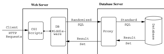
Fig. 3. SQLrand System Architecture
