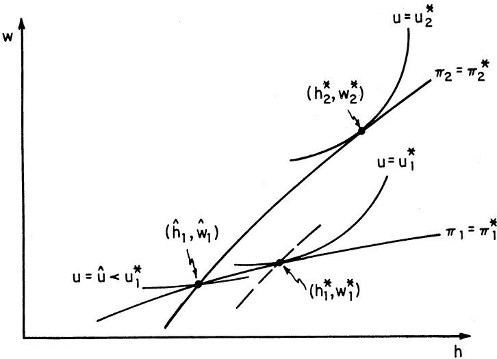
FIGURE III First-Best Equilibrium Not Implementable Second-best equilibrium characterized by inefficient underemployment in adverse state.
