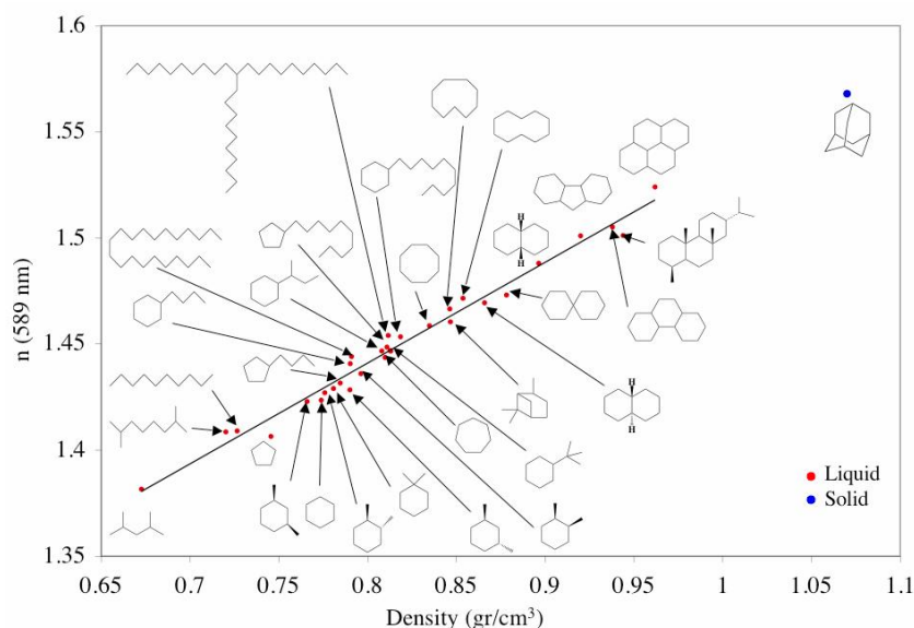
Fig. 1. Refractive index (d line) vs. density of alkanes and cycloalkanes at room temperature.
