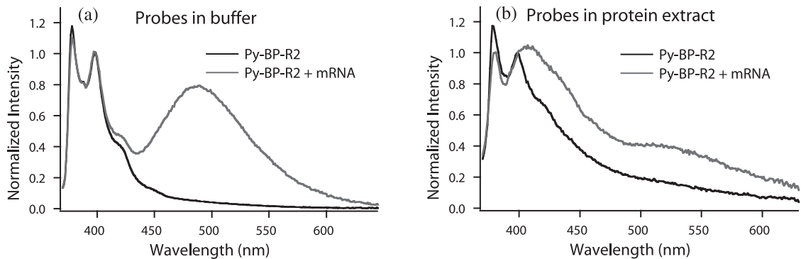
Figure 4. Steady-state fluorescence spectra of Py-BP-R2 in buffer solution (a) and cellular protein extract (b). [Py-BP-R2] = 0.1 \mu M; Buffer: 10 mM Tris (pH 7.5), 400 mM NaCl; hybridization time = 2 h; normalized at 400 nm.
