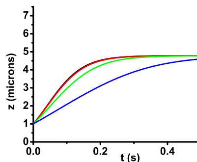
Fig. 6. Predicted stretching behavior of supercoiled DNA following a sudden force switch, as a function of the magnitude of the hydrodynamic drag induced by plectonemes. In this example, F_{\text{mag}} = 2.5 pN and \Delta Lk = +100 turns. The hydrodynamic drag opposing plectoneme removal corresponding to the simple model described in the text has been added in the equation of motion (1). Numerically solving this equation (red line) shows that this leads only to a nearly indistinguishable modification of the quasistatic dynamics (black line). However, traces generated by arbitrarily considering 10-fold (green line) and 50-fold (blue line) larger hydrodynamic drags are significantly different.
