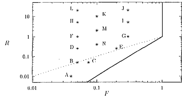
FIG. 2. The (R, F) parameter space, and the location of the runs discussed in this paper (cf. Table I). The dotted line is the line B=1 , i.e., L=L_R . The solid lines roughly indicate the boundary to whose right the SWE cease to apply.
