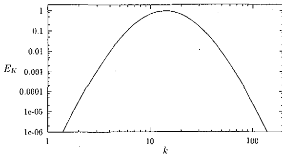
FIG. 1. Initial kinetic energy spectrum.
