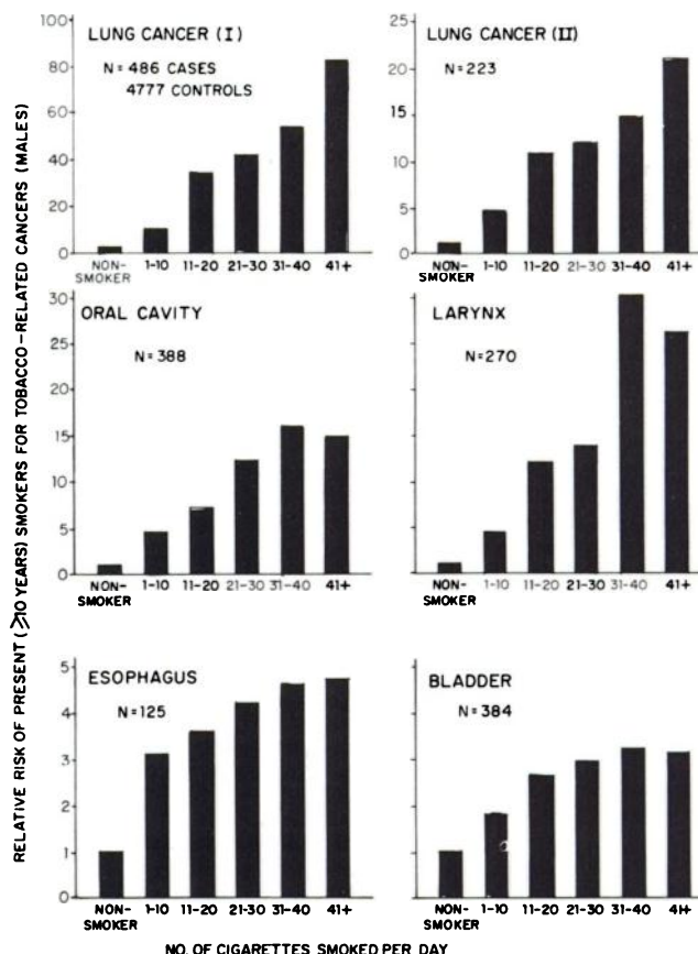
Chart 3. Relative risk of present (≥10 years) male smokers for tobacco-related cancers, by quantity smoked.
