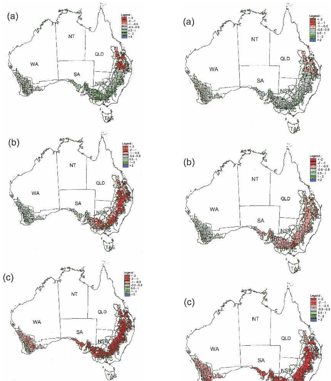
FIG. 2. Average standardized (relative to all years) shire wheat yield anomalies or impact FPs during EN years for (a) cluster-1 EN years (FP1), (b) cluster-2 EN years (FP2), and (c) cluster-3 EN years (FP3). Categories represent number of standard deviations of the average anomaly from the long-term mean.
