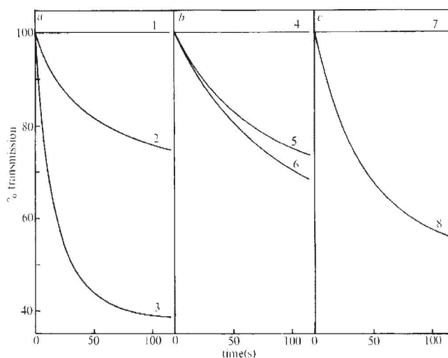
Fig. 1 The % transmission as a function of time for polystyrene latices. a , Curves for latices containing surface carboxylic acid groups: 1, no PEO added; 2, PEO of M_v = 4,000 added; 3, PEO of M_v = 23,000 added. b , Curves for latices stabilised by PAA: 4, no PEO added; 5, PEO of M_v = 4,000 added; 6, PEO of M_v = 23,000 added. c , Curves for latices stabilised by PEO: 7, no PAA added; 8, PAA of M_v = 19,300 added. Flocculant added at 20 p.p.m. in a and c and 50 p.p.m. in b .
