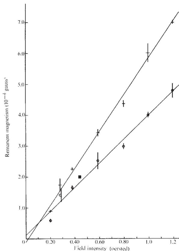
Fig. 2 Intensities of the control field and the remanences of the reconstituted sediment, before (+) and after ( \phi ) 100 oersted a.f. demagnetisation. Regression line slopes are 5.96 \pm 0.19 ( \times 10^{-4} gauss oersted ^{-1} ) and 3.87 \pm 0.20 ( \times 10^{-4} gauss oersted ^{-1} ), respectively. ■, Average remanent intensity of RC14-14, after 100 oersted a.f. demagnetisation 11 , plotted against the present axial dipole field intensity at the core site.
