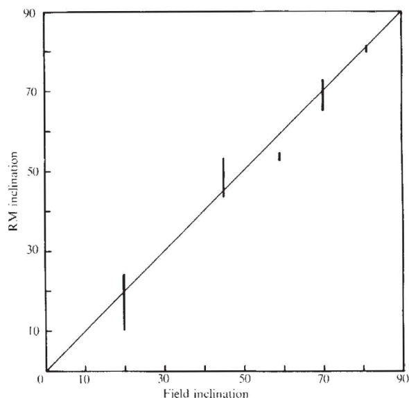
Fig. 1 Inclinations of the control field and the remanent magnetisation of the reconstituted sediment. Error bars represent range of remanent inclinations for each sample; the line of perfect agreement is shown. Successively steeper inclinations were produced in fields of 0.20, 0.38, 0.59 and 1.20 oersted, respectively.
