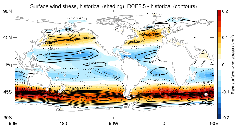
Figure 1. The historical (shading) and change (contours) from 1979–2005 to 2070–2099 in annual mean surface zonal wind stress evaluated as the multimodel mean of CMIP5 historical simulations and projections with the RCP85 high emissions scenario. The black circles denote the location of the maximum in climatological wind stress at each longitude in the historical period. The contour interval for the anomalies is 0.004 \text{ N/m}^2 with the zero line omitted. The models used are as in Simpson et al. [2014].
