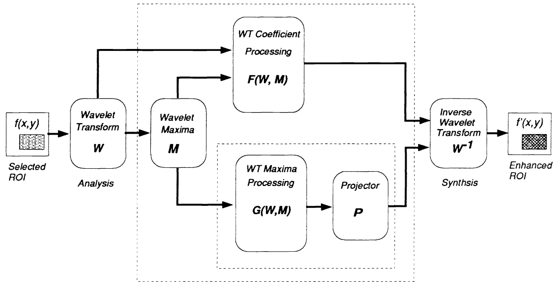
Figure 1. Processing structures for local feature enhancement by wavelet representations.
