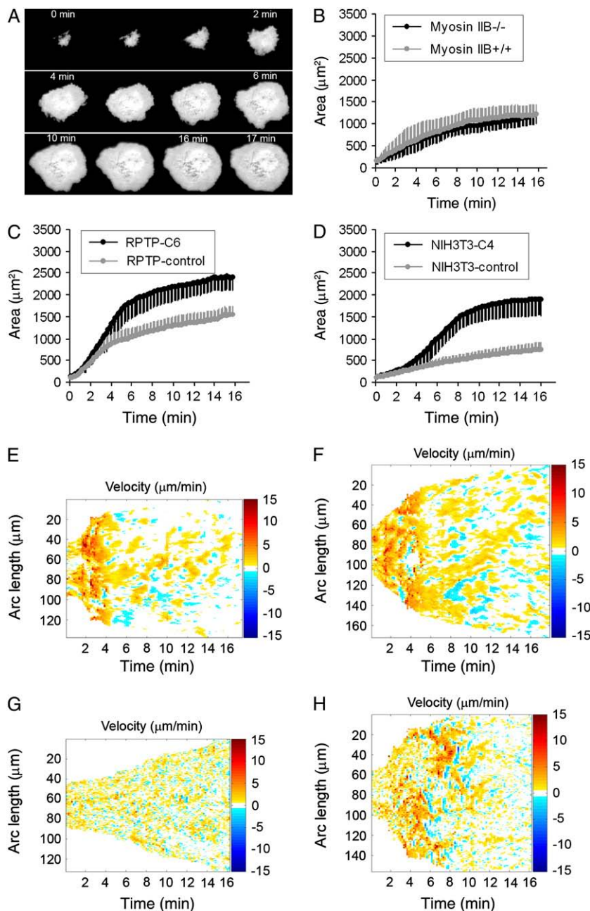
FIGURE 5 NMM-IIA regulates cell spreading of mouse embryonic fibroblasts. (A) Sequential TIRF images of a Calcein AM-labeled MEF cell spreading on fibronectin substrate. Panels B, C, and D are plots of cell area over a course of time. NMM-IIB +/+ and NMM-IIB -/- cells spread to similar areas on fibronectin substrate at early times (within 16 min) (B); RPTP-C6 cells spread significantly faster than RPTP-control cells (C); NIH3T3-C4 cells spread significantly faster than NIH3T3-control cells (D). Error bars show standard deviation. (E–H) are velocity maps as given by plotting velocity of protrusion/retraction of points at cell edge as a function of time and arc length (length of entire cell edge) that were obtained by analyzing 10-s interval time-lapse TIRF images of Calcein-AM labeled cells spreading on fibronectin at 37°C. Briefly, time-lapse image sequences were analyzed with Matlab to obtain a closed curve delineating the cell edge, which was then parameterized by arc length. For each point on the cell boundary in each frame of time-lapse sequential images, the normal velocity was calculated and displayed in color-coded plots. Points on the cell boundary are specified by time (in minutes) and arc length (in \mu\text{m} ); red coloring represents protrusion events, whereas blue represents retraction events as depicted by the velocity bars. Velocities with an absolute value < 0.5 \mu\text{m}/\text{min} were not considered to be relevant events. They are reflected as colorless patches among red and blue patches. Details are described in Materials and Methods section. Panels E, F, G, and H are representative samples of RPTP-control, RPTP-C6, NIH3T3-control, and NIH3T3-C4 cells, respectively.
