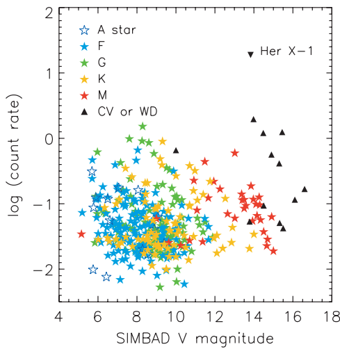
Figure 3. X-ray count rate vs. V for 139 known X-ray-emitting SIMBAD stars and 249 SIMBAD stars offset by <30'' from a RASS source. B was used for the two CVs and two WDs with no cataloged V .
