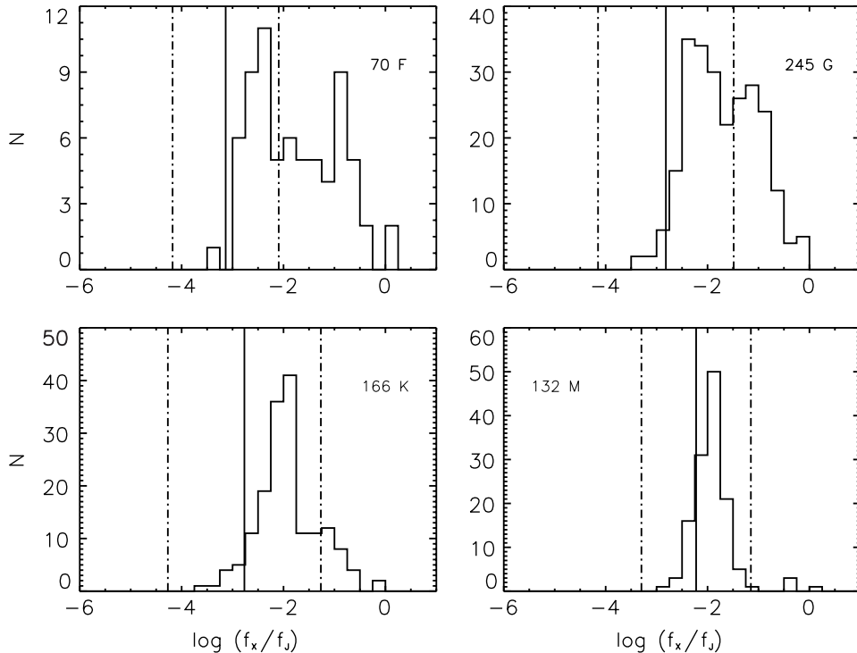
Figure 7. \log(f_x/f_J) ratios for the candidate SDSS counterparts with APO spectroscopy. The solid vertical lines correspond to the mean ( f_x/f_J ) and the dot-dashed vertical lines bracket the 2\sigma ( f_x/f_J ) range for each stellar type as derived from the RASS/SIMBAD sample. The number of SDSS/APO stars used to calculate these ( f_x/f_J ) ranges is indicated in each panel.
