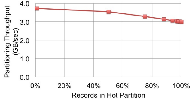
Figure 9: As the input data is increasingly skewed (i.e., unbalanced), the baseline accelerator’s throughput drops by up to 19% due to increased occurrence of back-to-back bursts to the same partition.
