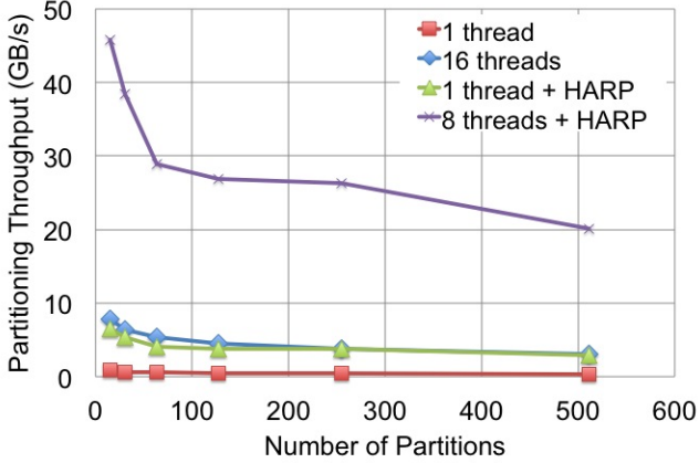
Figure 7: A single HARP unit outperforms single threaded software from 7.8X with 15 partitions to 9.0X with 511 partitions, matching the throughput of 16 threads.
