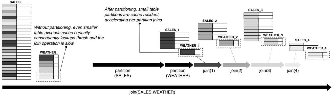
Figure 2: Joining two large tables easily exceeds cache capacity. State of the art join implementations, partition the tables to be joined then compute partition-wise joins, each of which exhibits substantially improved cache locality [28, 2]. Joins are extremely expensive on large datasets, and partitioning represents a significant fraction, up to half, of the observed join time [28].
