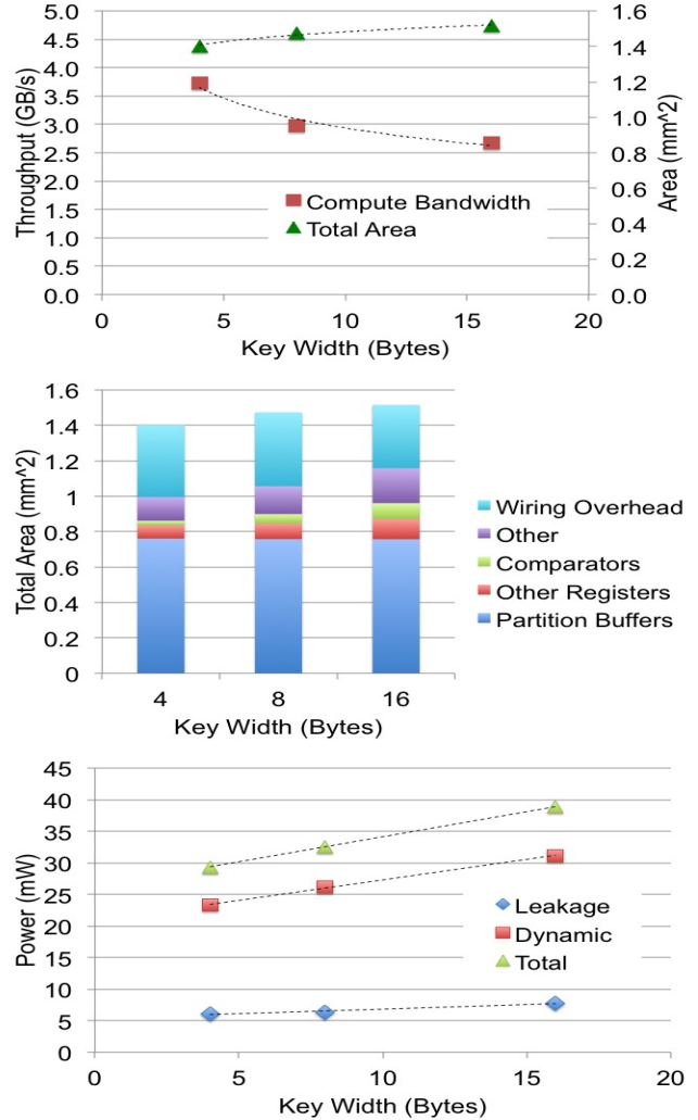
Figure 11: HARP throughput, area, and power at different maximum key widths.
