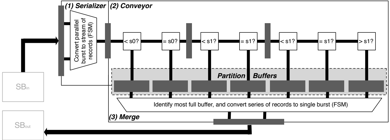
Figure 6: HARP draws records in bursts, serializing them into a single stream which is fed into a pipeline of comparators. At each stage of the pipeline, the record key is compared with a splitter value, and the record is either filed in a partition buffer (downwards) or advanced (to the right) according to the outcome of the comparison. As records destined for the same partition collect in the buffers, the merge stage identifies and drains the fullest buffer, emitting a burst of records all destined for the same partition.
