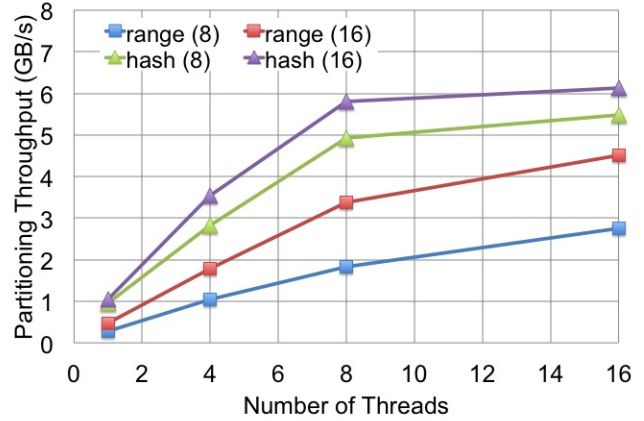
Figure 4: Partitioning bandwidth (in GB/sec of input) achieved for 128-way software partitioning using hash and range partitioning, as a function of the number of parallel threads. Data is shown for both 8 byte and 16 byte records.
