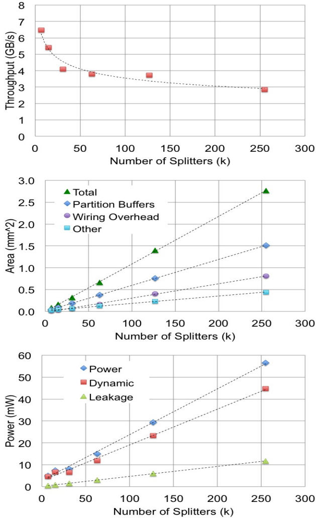
Figure 10: HARP throughput, area, and power for different numbers of splitters, creating a family of small to large HARP instances.
