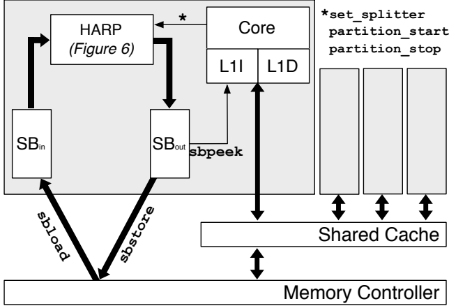
Figure 5: Block diagram of a HARP system architecture
