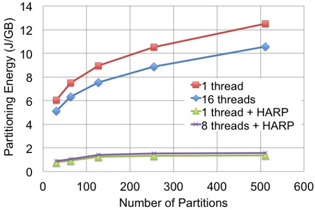
Figure 8: HARP-augmented cores partition data using 5.7-9.0X less energy than parallel or serial software.
