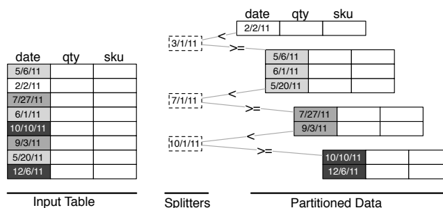
Figure 1: An example table of sales records range partitioned by date, into smaller tables. Processing big data one partition at a time makes working sets cache-resident, dramatically improving the overall analysis speed.
