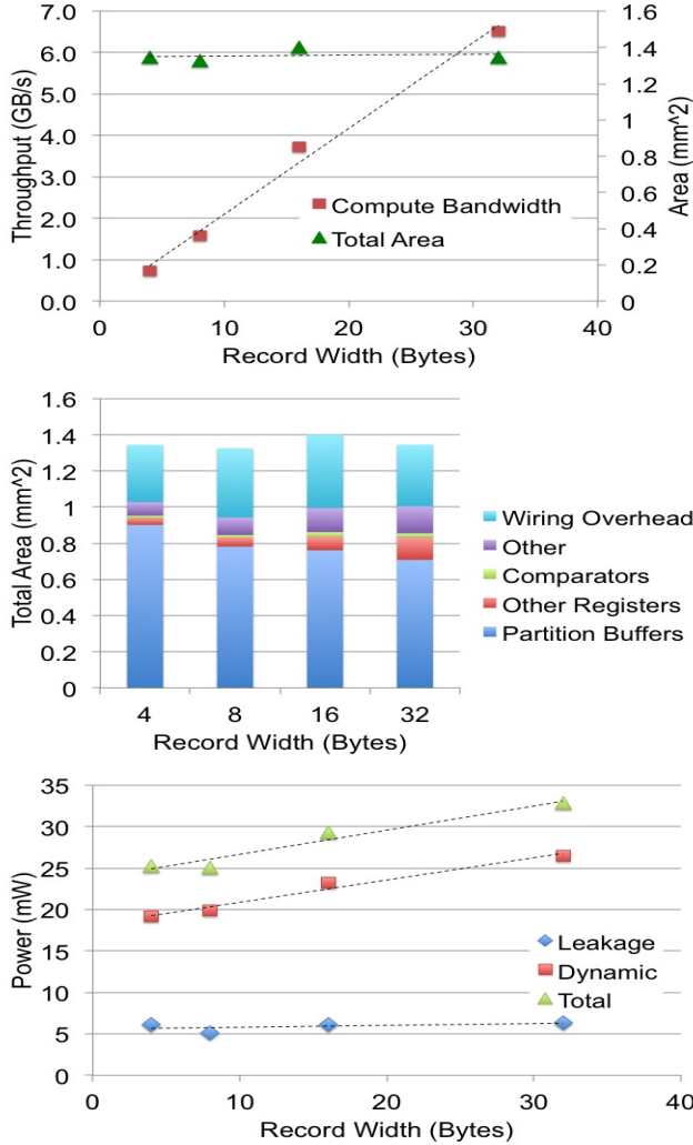
Figure 12: HARP throughput, area, and power at different maximum record widths.
