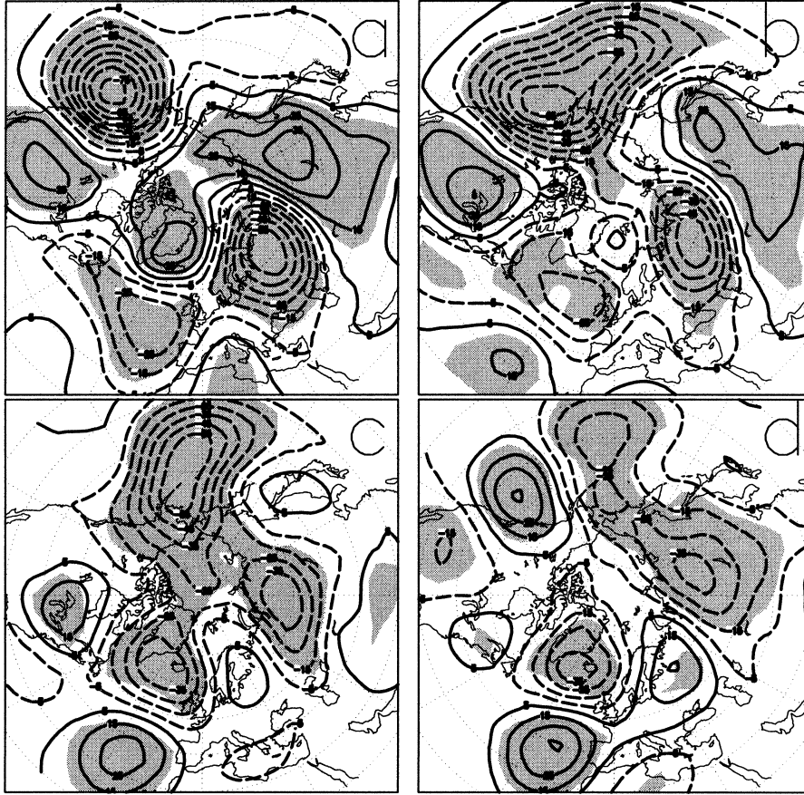
FIG. 5. Composite anomalies of Z_{700} maps from the IS time series keyed to the 20–30-day signal of NH mountain torque: (a) 0-day lag, (b) 3-day lag, (c) 6-day lag, and (d) 9-day lag. Contour interval: 10 m; positive values, heavy solid; negative values, heavy dashed; 95% confidence, shaded; continental contours, light solid. The days for each composite cycle are counted from the local extremum of the 20–30-day NH T_M for that cycle (see text for details).
