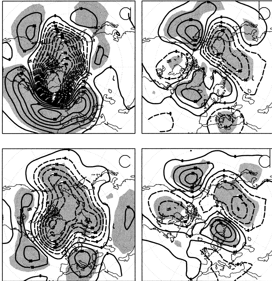
FIG. 9. Composite anomalies of the IS Z_{700} maps keyed to (a), (b) the 20–30-day NH PC-2 and (c), (d) the 20–30-day planetary angular momentum M_n : (a), (c) 0-day lag and (b), (d) 6-day lag. Same conventions and parameters as in Fig. 5.
