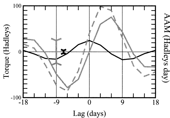
FIG. 6. Composites of different terms in the AAM budget during the composite cycle illustrated in Fig. 5: IS NH T_M (black solid); integral of IS NH T_M (gray solid); and global IS M (gray dashed). Units for the global atmospheric angular momentum M are in hadley day: 1 \text{ H d} = 8.64 \times 10^{22} \text{ kg m}^2 . The vertical black bar and the vertical gray bar indicate the 95% confidence interval of a Monte Carlo test for the torque and for the global AAM, respectively.
