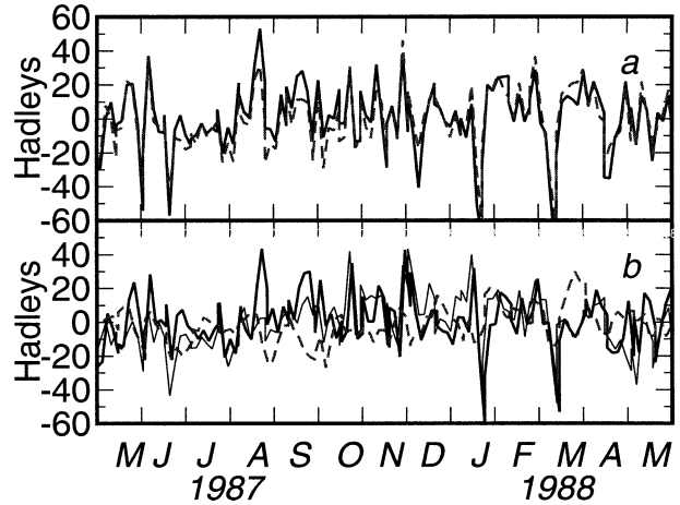
FIG. 1. Atmospheric angular momentum balance and torques over one year. (a) Global AAM tendency (heavy solid) and total torque (dashed); (b) global mountain torque (heavy solid), frictional torque (dashed), and Northern Hemisphere mountain torque (light solid).
