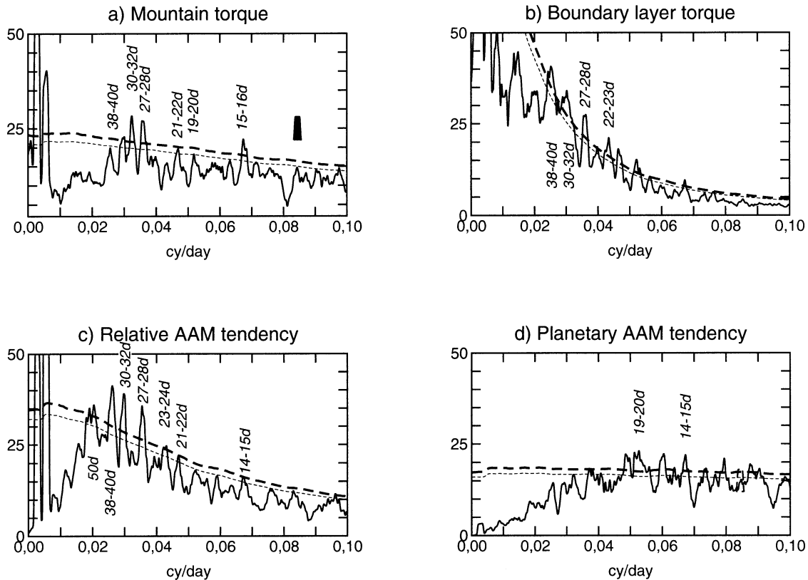
FIG. 3. (a)–(d) Spectra of the different terms in the AAM budget; see Eqs. (2)–(8). All curves are normalized by the mountain torque variance with annual cycle subtracted. The spectra (solid curve) are obtained by taking the Fourier transform of the 3d series, and by smoothing the resulting periodogram with a 33% cosine 30-point window [shown as the filled curve in (a)]. This window yields a frequency resolution of 2.3 \times 10^{-3} cycles per day. The heavy and light dashed lines show the 99% and 95% significance level of a Monte Carlo test based on the spectra of 100 realizations of an AR-1 process whose variance and lag-1 autocorrelation were least squares-fitted to the 3d series with annual cycle subtracted.
