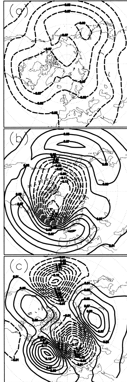
FIG. 7. NH EOFs of the 700-hPa geopotential height field: (a) EOF-1, (b) EOF-2, and (c) EOF-5.
