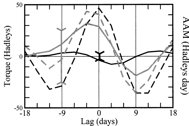
FIG. 10. Composites of different terms in the IS AAM budget keyed to the 20–30-day cycle of the Arctic Oscillation (PC-2 in our analysis): NH T_M (black solid), integral of NH T_M (gray solid), global AAM M (gray dashed), and planetary AAM (black dashed). Same conventions and parameters as in Fig. 6.
