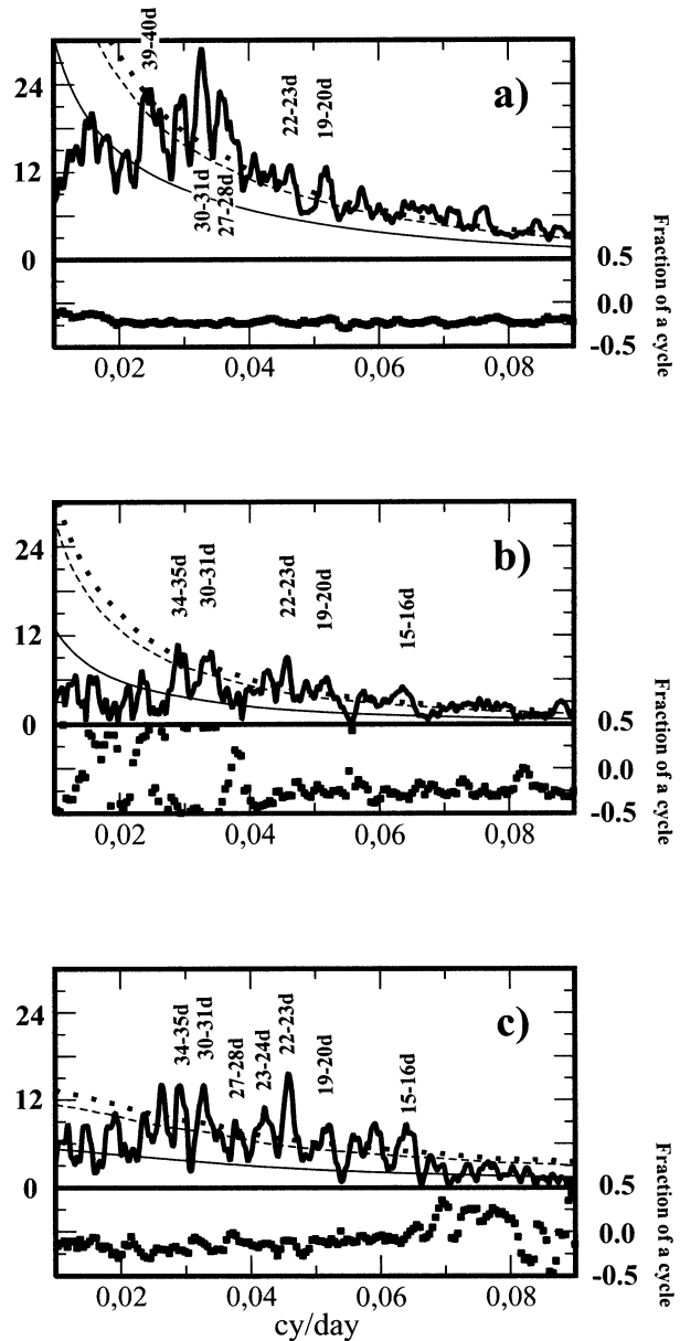
FIG. 8. Cross-spectra between NH T_M and the leading NH PC- s : (a) NH T_M vs NH PC-1, (b) NH T_M vs NH PC-2, and (c) NH T_M vs NH PC-5. Upper part of panels: cross-spectral amplitude (heavy solid) with 99% confidence level (heavy dots), 95% confidence level (light dashed), and median (light solid) of Monte Carlo test. Lower panels: phase difference (filled squares). The cross-spectra are computed from the cross periodogram of the 3d series smoothed with the same window as shown in Fig. 3a. All cross-spectral amplitudes are normalized by the NH- T_M and PC standard deviation with annual cycle subtracted. For each PC and torque series, the Monte Carlo test uses 100 cross-spectra of AR-1 bivariate series that fit the 3d series of NH T_M and of the corresponding PC, with annual cycle subtracted.
