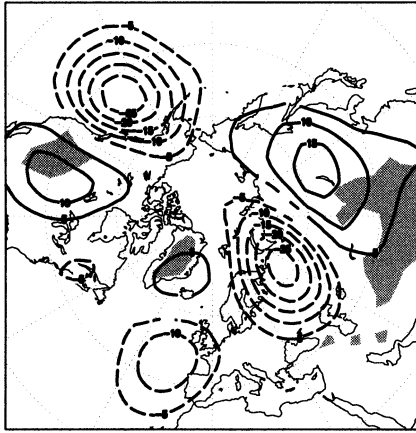
FIG. 2. The 700-hPa geopotential height field regression with respect to the NH mountain torque in the intraseasonal band; altitudes above 1500 m are shaded. Positive contours are solid, negative ones are dashed; contour interval is 5 m. See Figs. 2a,b in Part II for the corresponding regressions with respect to the Rockies and the Himalayas torques, separately.
