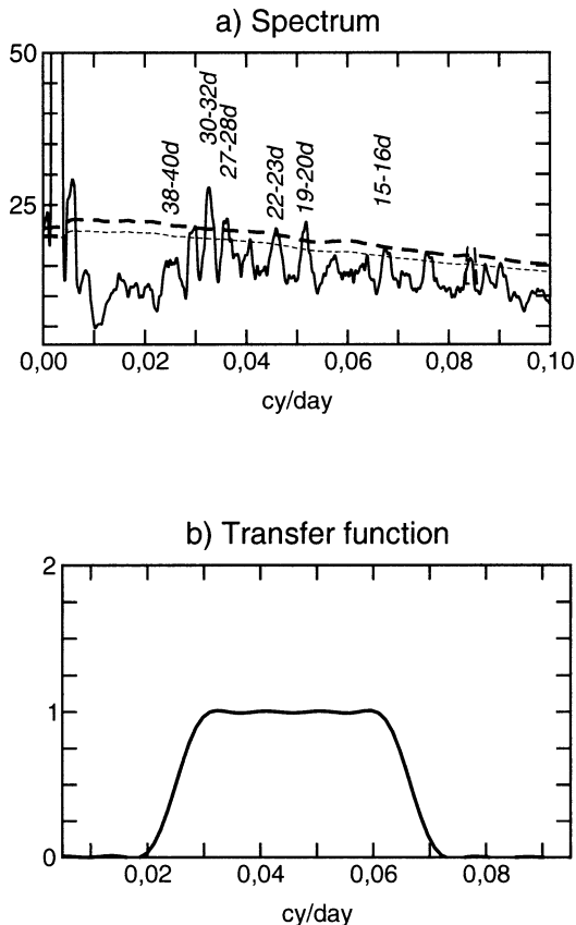
FIG. 4. NH mountain torque. (a) Spectrum of the 3d series, same parameters and normalization as in Fig. 3; (b) transfer function of the bandpass filter used to extract the 20–30-day series.
