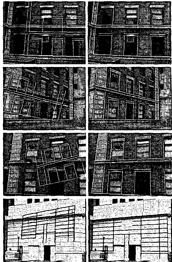
Figure 6: Pose estimation at locations 1 through 4: Each pair shows the model projected on the image using the initial pose of the camera (left), and the resulting pose of the camera (right) for the corresponding test location.
