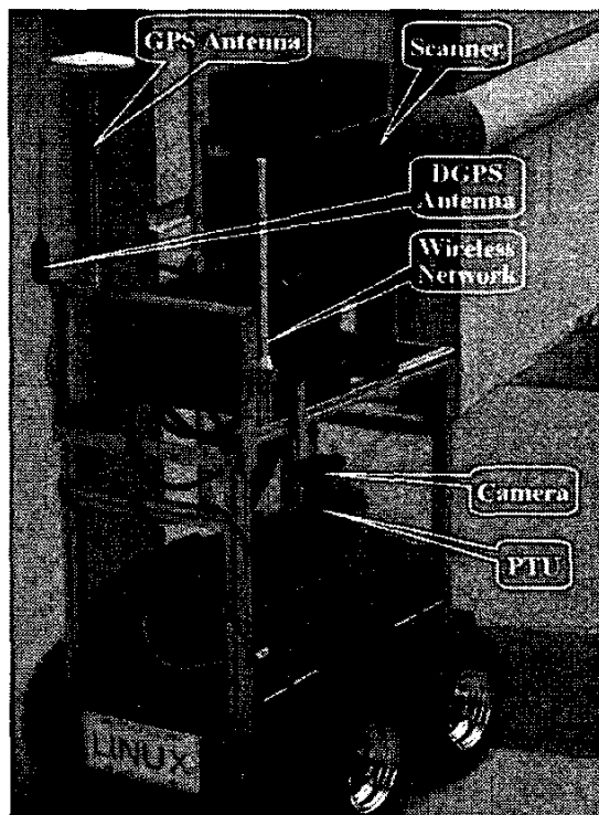
Figure 1: Mobile robot for automated site modeling
