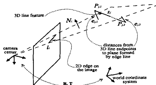
Figure 2: Error metric used for pose estimation
