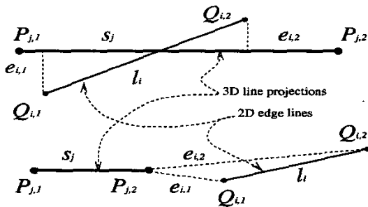
Figure 3: Distance metric used for matching.
