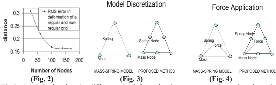
Fig.2. A graph showing the difference in deformation between a regular and an irregular mesh connectivity. Fig.3. A schematic representation of a discrete 3D model using the proposed approach and the corresponding representation using a mass-spring model.[7] Fig.4. A schematic representation of force application in the proposed approach as well as in the mass-spring model.
