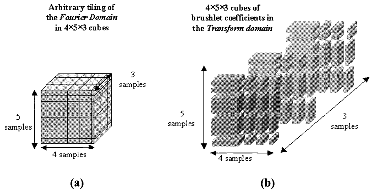
Figure 5: (a) 3D tiling of the Fourier domain with arbitrary sampling along each direction. (b) Corresponding structure of brushlet coefficients in the transform domain.
