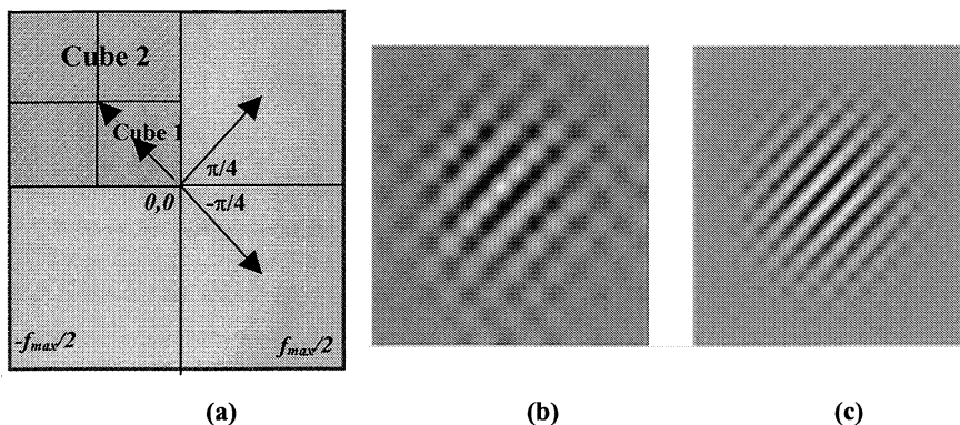
Figure 2: Illustration in 2D of the influence of the tiling of the Fourier domain on the resolution and orientation of a brushstrokes. (a) Tiling of the Fourier domain. (b) Real-Part of coefficient for Cube 1. (c) Real-Part of coefficient for Cube 2.
