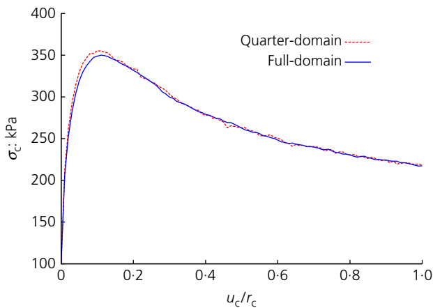
Fig. 3. Cavity pressure against normalised cavity expansion displacement
