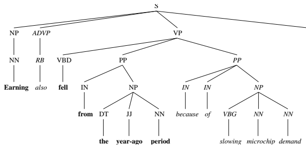
Figure 1: Penn Treebank tree with adjuncts in italic.
