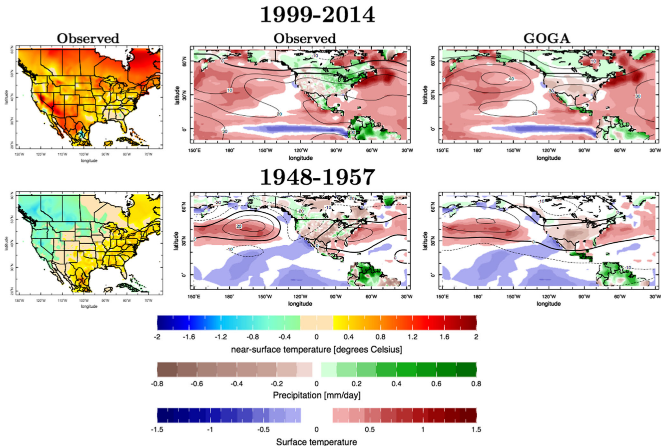
Fig. 3 Anomalies of the observed surface air temperature (left), observed SST over ocean, precipitation over land and 200 mb heights (middle) and observed SST over ocean, modeled ensemble mean precipitation
