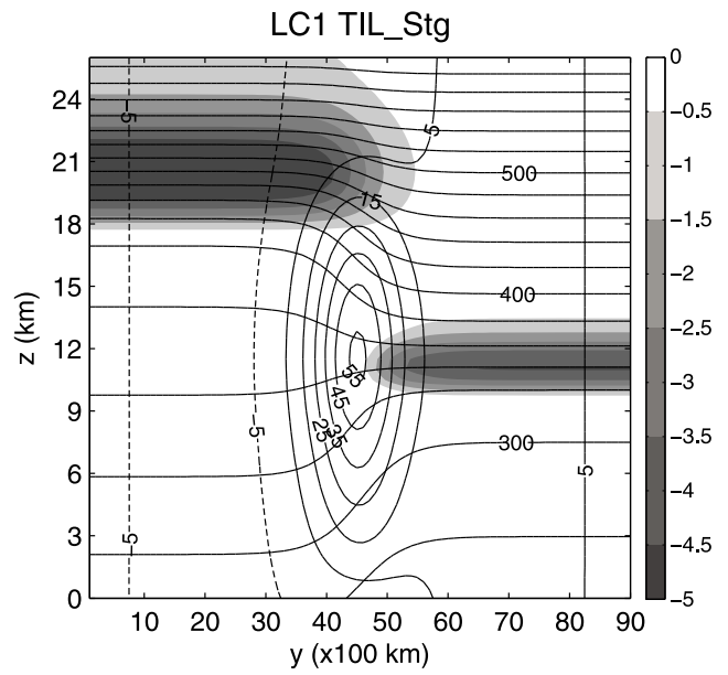
Figure 9. As in Figure 2d, but with an additional barotropic and anticyclonic wind shear, with an amplitude of 10 \text{ m s}^{-1} (see section A3 for details), to generate an LC1 life cycle.
