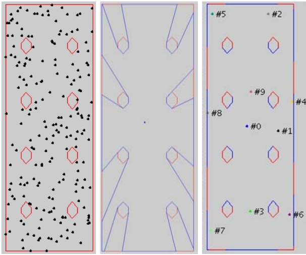
Fig. 2. The initial simulated test region for the first phase of our view planning algorithm together with an initial set of 200 viewpoints randomly distributed throughout the free space of the region (left). The unclipped visibility polygon of one of the potential views (center). The final set of 10 scanning locations chosen for our simulated test region, with the clipped obstacle edges for scanning location #0 indicated in blue (right). All the figures in this paper should be viewed in color.
