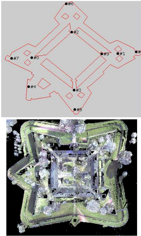
Fig. 4. On the top are the viewing locations chosen by the initial modeling phase for the outer courtyard of Fort Jay. On the bottom is the entire model of Fort Jay (seen from above) generated by the initial planning stage for the inner and outer courtyards and the moat.
