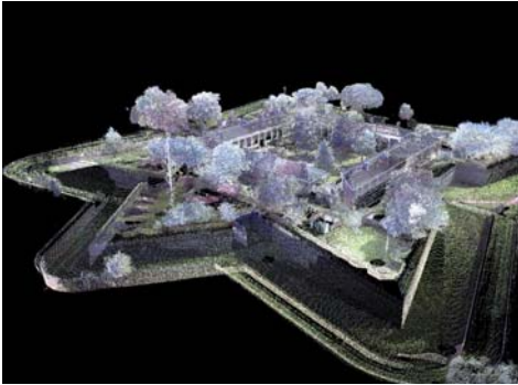
Fig. 8. A view of the final model of Fort Jay after all 34 scans from phases one and two were acquired.
