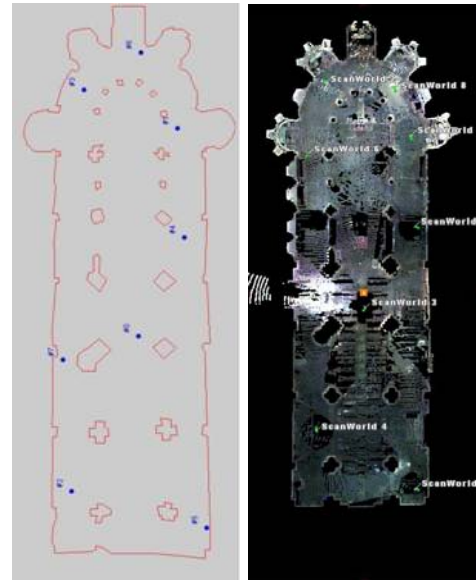
Fig. 3. On the left is the 2-D map of Saint Menoux’s interior. Also shown are the 8 scan locations determined by the initial two-dimensional view planner using a grazing angle constraint of 70^\circ . On the right is a slice taken at floor level of the complete model acquired after taking all 8 scans.
