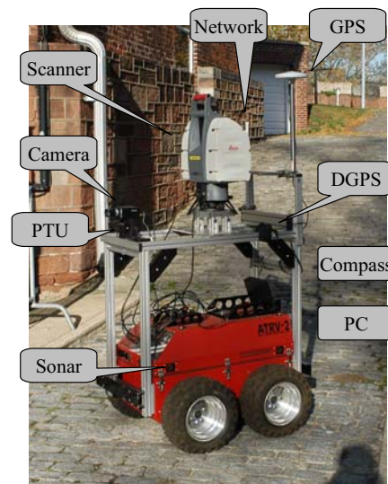
Fig. 1. The ATRV-2 AVENUE Based Mobile Robot.
