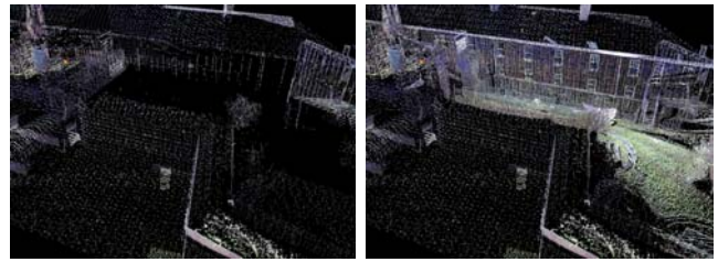
Fig. 6. On the left is a segment of the model of Fort Jay created during phase one of the algorithm. The hole in the left figure is caused by an unpredicted occlusion of one of the initial scanning locations. On the right is the same section of the model after the first two NBVs from phase two were computed and acquired.
