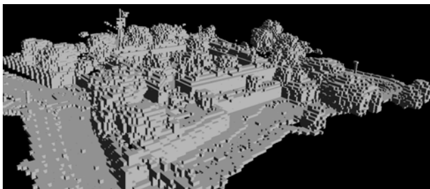
Fig. 5. A representation of the seen-occupied cells of Fort Jay's voxel grid. It was constructed at the end of phase one from the point cloud acquired in section IV-A.2.
