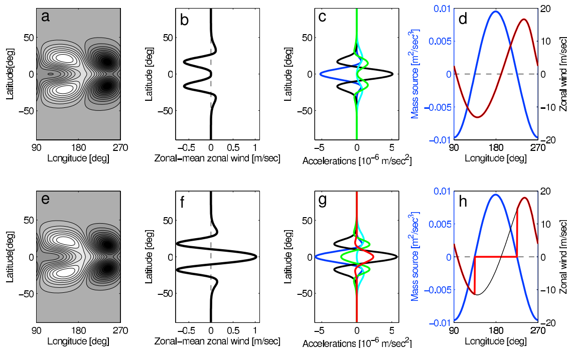
Figure 1. (top) A solution with \mathbf{R} = 0 and (bottom) an otherwise identical solution with \mathbf{R} given by equation (3). (a, e) Geopotential gh . (b, f) Zonal-mean zonal wind \bar{u} . (c, g) Accelerations of the zonal-mean zonal wind in the equilibrated state (see text). (d, h) Mass source Q at the equator (blue), zonal wind at the equator ( thin black ), and zonal wind at the equator that is advected into ( Q > 0 ) or out of ( Q < 0 ) the layer (red). Figures 1a, 1d, and 1e and 1h show only half the domain (longitudes 90^\circ to 270^\circ ) for clarity. Both cases adopt \tau_{\text{rad}} = \tau_{\text{drag}} = 5 days, \phi_0 = 0^\circ , gh_0 = 4000 \text{ m}^2 \text{ sec}^{-2} (as given by Gill [1980]), and forcing amplitude gS_0 = 0.0098 \text{ m}^2 \text{ sec}^{-3} .
