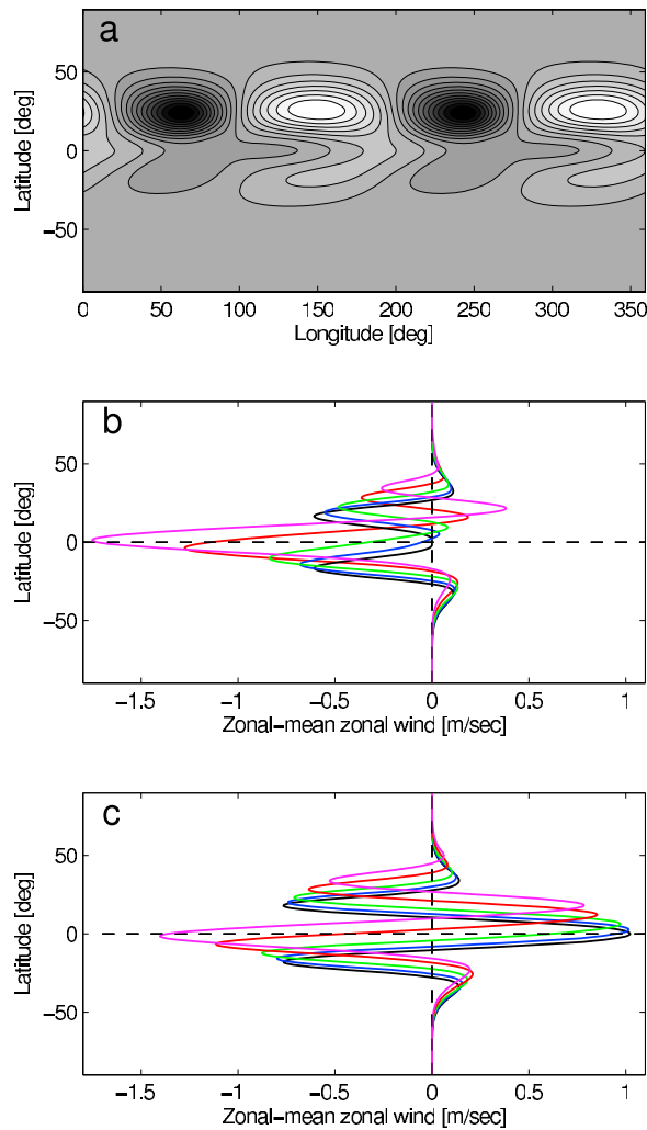
Figure 2. (a) Geopotential for a case identical to that in Figure 1 (top) except that the peak in heating is displaced 10^\circ latitude north of the equator. (b) Zonal-mean zonal wind for a sequence of solutions with \mathbf{R} = 0 (as in the standard Matsuno-Gill problem) and \phi_0 = 0^\circ (black), 2^\circ (dark blue), 5^\circ (green), 10^\circ (red), and 15^\circ (magenta). (c) Identical to Figure 2b but for a sequence of simulations with \mathbf{R} given by equation (3).
