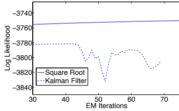
Figure 1: a) The training log likelihood when the Kalman filtering is one step from divergence b) Results for EM training
