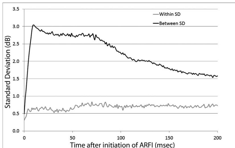
FIGURE 4. Plot of standard deviations within and between triplicate ARFI exposures at 10 sites linearly spaced at 0.1-mm intervals. The response to ARFI was highly reproducible in multiple exposures for any single spot, but varied considerably between spatial positions.
