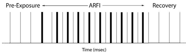
FIGURE 1. Schematic illustration of ultrasound emission pattern. With the ultrasound beam fixed along one line of sight, single cycles of 18-MHz center frequency are emitted at 1-ms intervals. After each pulse, echo data from the posterior of the eye are received in under 0.05 ms. After 100 such pulse/echo events have established baseline conditions, a 0.25-ms long (4500 cycles), 18-MHz tone burst is emitted instead of a monocycle. This produces significant radiation force and interferes with echo data (since the tone burst is longer than pulse/echo transit time), creating a marker indicating start of ARFI exposure. Nine additional tone bursts interleaved between monocycles are then emitted, generating radiation force, but leaving sufficient time after each monocycle to receive echo data without interference. Subsequent to this, the system returns to monocycles at 1-ms intervals, allowing assessment of postexposure recovery.
