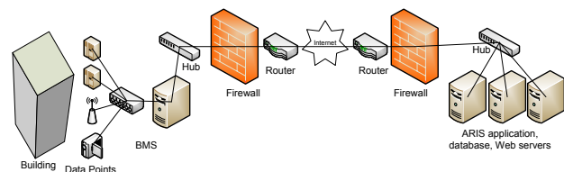
Figure 6. Experimental setup.
