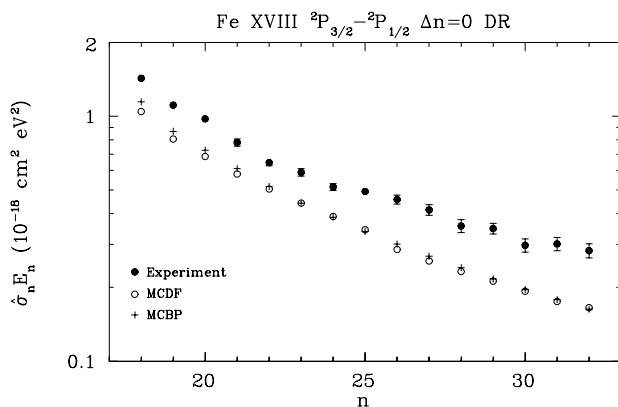
FIG. 6.—DR resonance strength \hat{\sigma}_n E_n as a function of the principal quantum number n for Fe XVIII to Fe XVII \Delta n = 0 DR via the {}^2P_{3/2}-{}^2P_{1/2} core excitation. There is an estimated \leq 20\% total systematic uncertainty in our experimental values (at a 90% confidence level). Filled circles are the present experimental results. Error bars represent the 1\sigma statistical fitting uncertainties. Open circles are our MCDF calculations and crosses are our MCBP calculations.
