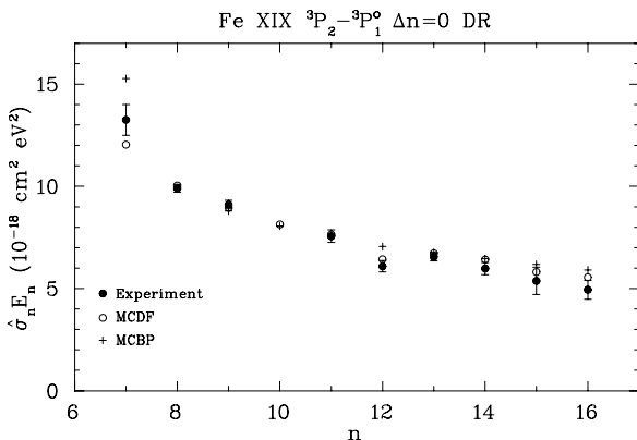
FIG. 11.—DR resonance strength \hat{\sigma}_{n,n} E_n as a function of the principal quantum number n for Fe XIX to Fe XVIII \Delta n = 0 DR via the ^3P_2-^3P_1 core excitation. See Fig. 6 for further details.
