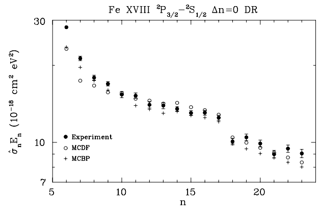
FIG. 7.—DR resonance strength \hat{\sigma}_n E_n as a function of the principal quantum number n for Fe XVIII to Fe XVII \Delta n = 0 DR via the {}^2P_{3/2}-{}^2S_{1/2} core excitation. See Fig. 6 for further details.
