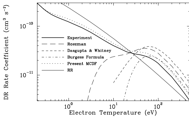
FIG. 5.—Fe XIX to Fe XVIII Maxwellian-averaged \Delta n = 0 DR rate coefficients. The thick solid line is calculated using the measured DR resonance strengths and energies extracted from the results shown in Fig. 2 and listed in Table 4. There is an estimated \lesssim 20\% total systematic uncertainty in our experimentally inferred rate. Also shown are existing theoretical calculations by Roszman (1987b; long-dashed curve ) and Dasgupta & Whitney (1994; short-dashed curve ), the Burgess formula (Burgess 1965; short-dashed-dotted curve ), and our new MCDF calculations ( dotted curve ). Our MCBP rate (not shown here) agrees well with our MCDF rate. The thin solid curve shows the recommended RR rate of Arnaud & Raymond (1992).
