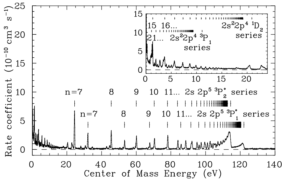
FIG. 2.—Measured Fe XIX to Fe XVIII recombination rate coefficient vs. electron-ion collision energy. \Delta n = 0 DR resonances resulting from {}^3P_2-{}^3P_1 , {}^3P_2-{}^1D_2 , {}^3P_2-{}^3P_2^o , and {}^3P_2-{}^3P_1^o core excitations are labeled for capture into high l levels. The nonresonant “background” rate is due primarily to RR with some residual CT (see text).
