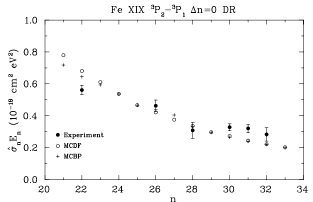
FIG. 8.—DR resonance strength \hat{\sigma}_n E_n as a function of the principal quantum number n for Fe XIX to Fe XVIII \Delta n = 0 DR via the {}^3P_2-{}^3P_1 core excitation. See Fig. 6 for further details.
