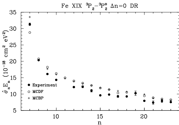
FIG. 10.—DR resonance strength \hat{\sigma}_{n,n} E_n as a function of the principal quantum number n for Fe XIX to Fe XVIII \Delta n = 0 DR via the ^3P_2-^3P_2 core excitation. See Fig. 6 for further details.
