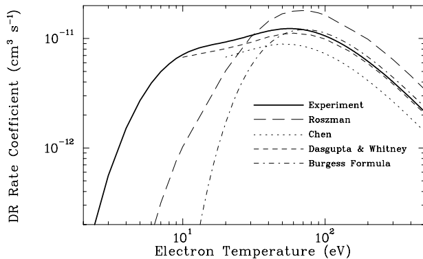
FIG. 3.—Fe XVIII to Fe XVII Maxwellian-averaged rate coefficients for \Delta n = 0 DR via ^2P_{3/2} - ^2S_{1/2} core excitations. The thick solid line is the integration of the experimental DR resonance strengths and energies extracted from the results shown in Fig. 1 and listed in Table 3. There is an estimated \lesssim 20\% total systematic uncertainty in our experimentally inferred rate. Calculations are from Roszman (1987a; long-dashed curve), Chen (1988; dotted curve), Dasgupta & Whitney (1990; short-dashed curve), and the Burgess formula (Burgess 1965; short-dash-dotted curve).
