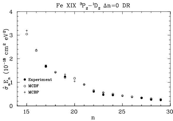
FIG. 9.—DR resonance strength \hat{\sigma}_{n,n} E_n as a function of the principal quantum number n for Fe XIX to Fe XVIII \Delta n = 0 DR via the ^3P_2-^1D_2 core excitation. See Fig. 6 for further details.
