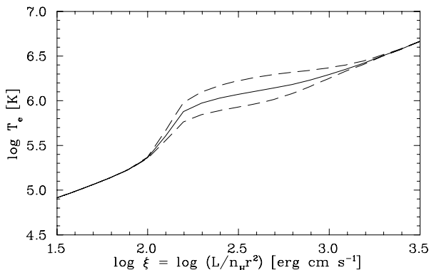
FIG. 12.—Predicted electron temperature vs. ionization parameter \xi for a model AGN ionizing spectrum illuminating a slab of gas with cosmic abundances. The solid curve shows the predicted T_e using our inferred Fe xviii and Fe xix DR rates and the unchanged \Delta n = 0 DR rates for Fe xx through Fe xxiv. The upper (lower) dashed curve results when the \Delta n = 0 DR rates for Fe xx through Fe xxiv are increased (decreased) by a factor of 2.
