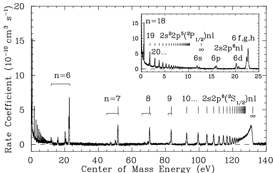
FIG. 1.—Measured Fe XVIII to Fe XVII recombination rate coefficient vs. electron-ion collision energy. \Delta n = 0 DR resonances resulting from {}^2P_{3/2} - {}^2P_{1/2} and {}^2P_{3/2} - {}^2S_{1/2} core excitations are labeled. The nonresonant “background” rate is due primarily to RR with some residual CT (see text).
