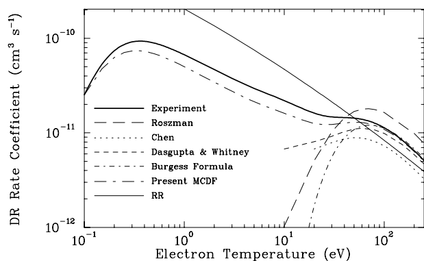
FIG. 4.—Fe XVIII to Fe XVII Maxwellian-averaged \Delta n = 0 DR total rate coefficients. The thick solid curve is the integration of the experimental DR resonance strengths and energies extracted from the results shown in Fig. 1 and listed in Tables 2 and 3. There is an estimated \lesssim 20\% total systematic uncertainty in our experimentally inferred rate. Existing calculations by Roszman (1987a; long-dashed curve ), Chen (1988; dotted curve ), Dasgupta & Whitney (1990; short-dashed curve ), and the Burgess formula (Burgess 1965; short-dash-dotted curve ) do not include the ^2P_{3/2} \rightarrow ^2P_{1/2} DR channel. The long-dash-dotted curve shows the results of our new MCDF calculations which include this channel. Our MCDF rate (not shown here) agrees well with our MCDF rate. The thin solid curve shows the recommended RR rate of Arnaud & Raymond (1992).
