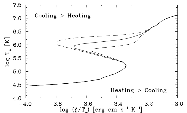
FIG. 13.—Predicted electron temperature vs. \xi/T_e for a model AGN ionizing spectrum illuminating a slab of gas with cosmic abundances. The solid curve shows the predicted T_e using our inferred Fe xviii and Fe xix DR rates and the unchanged \Delta n = 0 DR rates for Fe xx through Fe xxiv. The upper (lower) dashed curve results when the \Delta n = 0 DR rates for Fe xx through Fe xxiv are increased (decreased) by a factor of 2.
