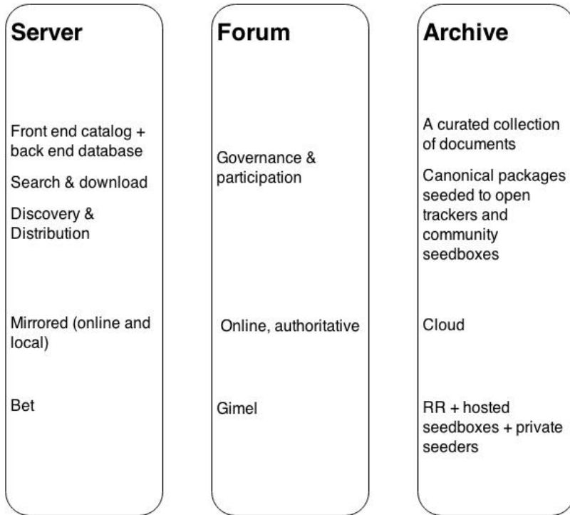
Figure 3: Aleph's anatomy
